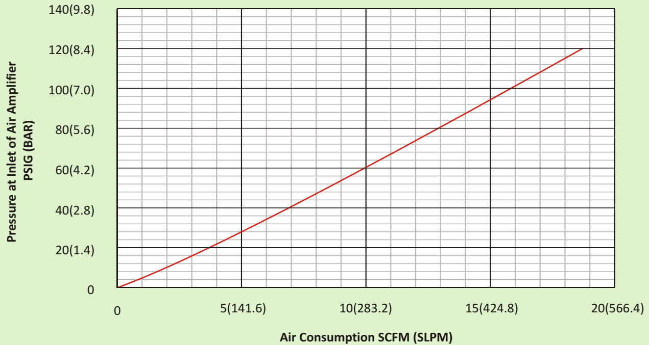
Pressure vs. Air Consumption for Model 40001 & 40001S Adjustable Air Amplifier
